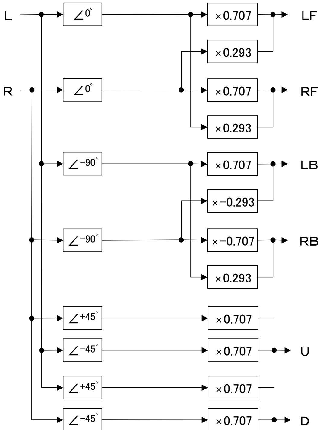
6 Channel Decoder
