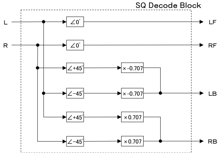
SQ Decode Block Diagram (improved symmetry)
