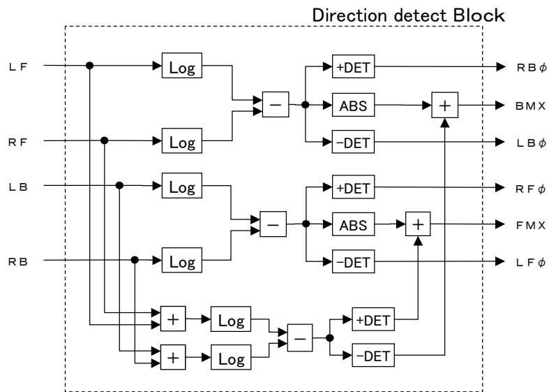
Sound source detection Block Diagram
