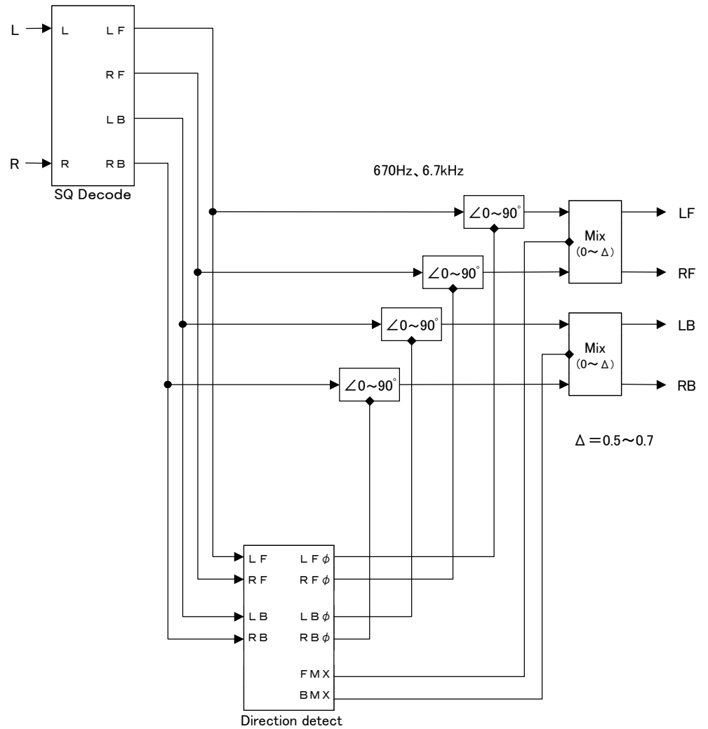
SQ Full Logic Decoder Block Diagram
