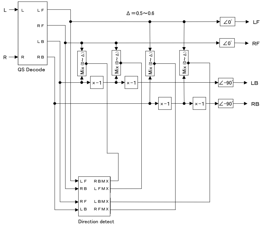
QS Full Logic Decoder Block Diagram
