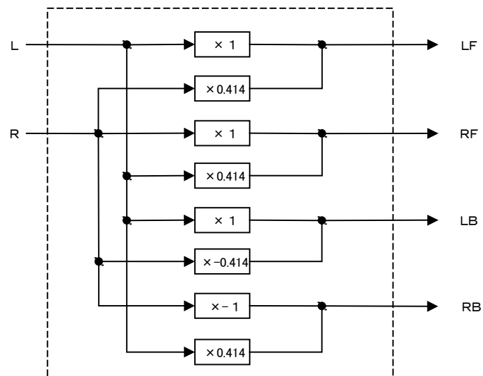
QS Decode Block Diagram
