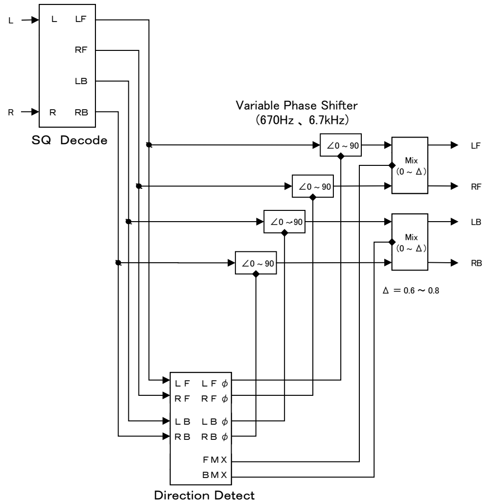
SQ Full Logic Decode Block Diagram
