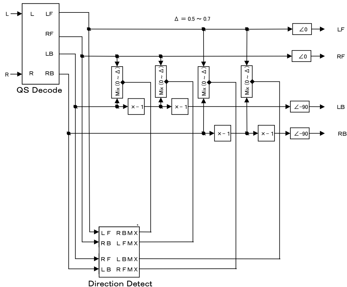
QS Full Logic Decode Block Diagram
