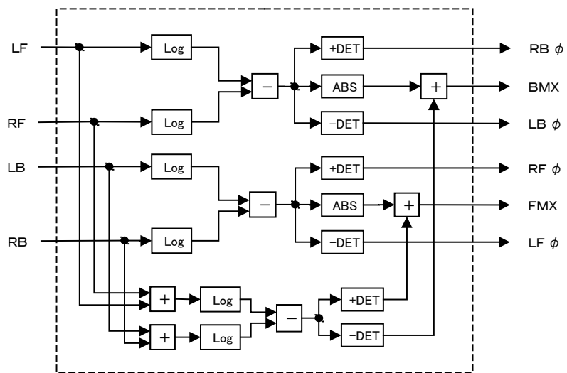
Direction Detect Block Diagram
