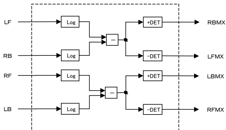
Direction Detect Block Diagram
