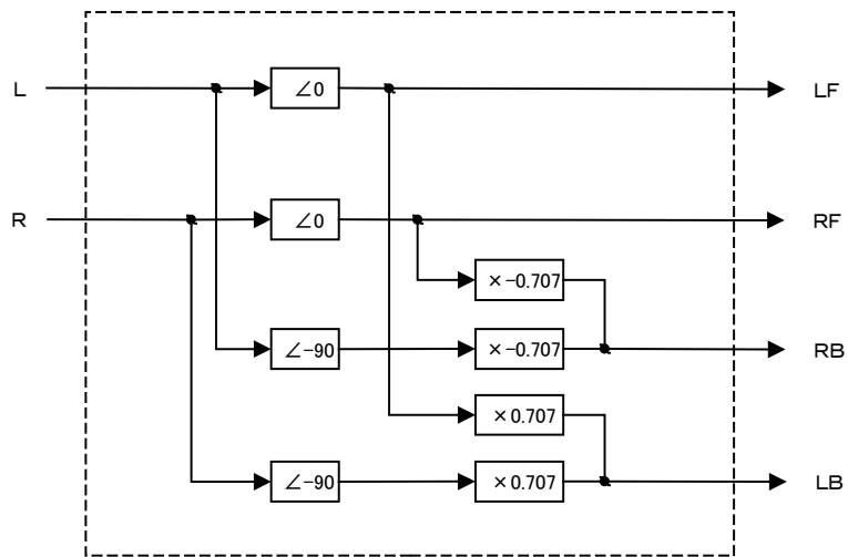
SQ Decode Block Diagram
